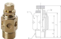
MODEL [ØD-T] Tube(Metric) – Thread(R)
