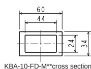
KBA-10-FD-M** cross section
