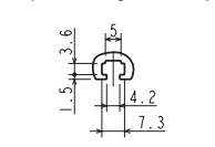
T groove: B (For M4 hexagon nut)
