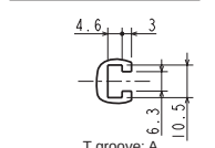
T groove: A (For M6 hexagon head bolt)
