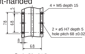
Z-axis slider details
