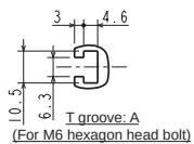
T groove: A (For M6 hexagon head bolt)
