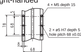
Z-axis slider details
