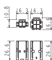
Motor/brake connector
