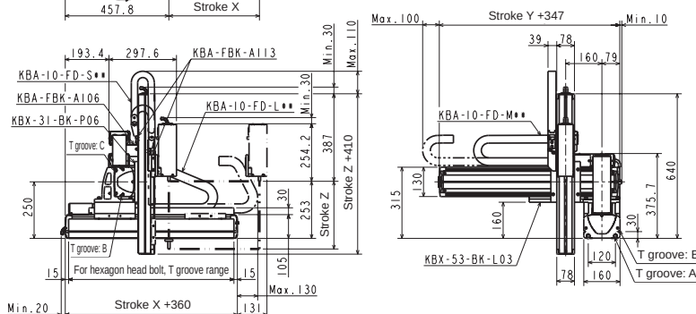
KBA-10-FD-M**cross section KBA-10-FD-S**cross section
