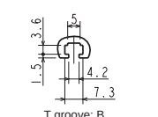
T groove: B (For M4 hexagon nut)
