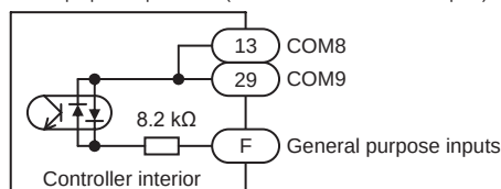
General purpose input circuit (common to NPN and PNP inputs)
