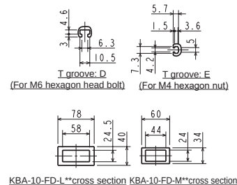
KBA-10-FD-L**cross section KBA-10-FD-M**cross section
