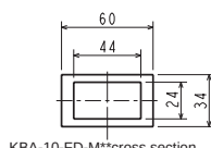
KBA-10-FD-M** cross section
