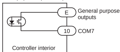
General purpose output circuit (common to NPN and PNP outputs)
