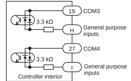
General purpose input circuit (common to NPN and PNP inputs)
