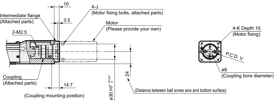
Motor Mounting Section Detail Drawing
