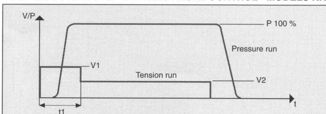
CHARACTERISTICS OF THE ELECTRICAL CONTROL - MODELS KK
